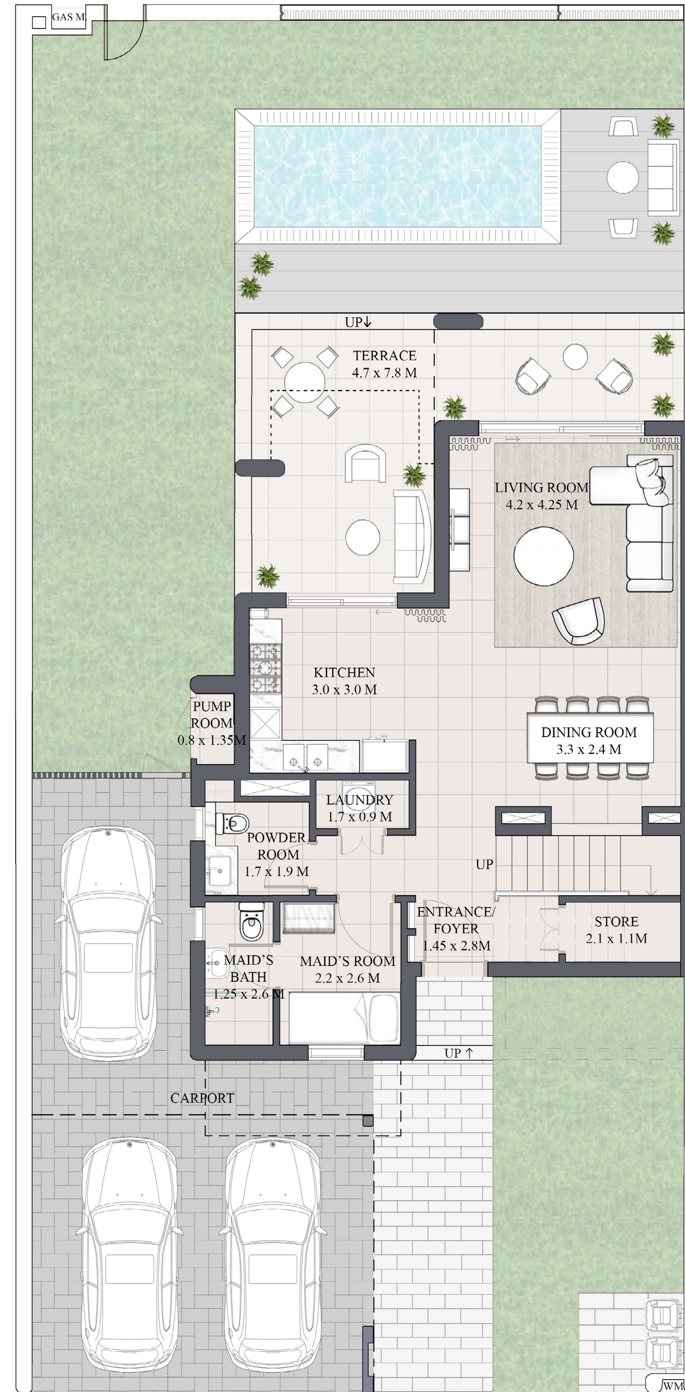
GROUND FLOOR
